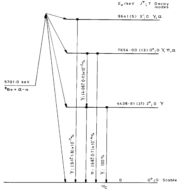
Figure 4.6. – Energy level diagram for {}^{12}\text{C} indicating electromagnetic transitions. Extracted from [125], based on [127].
