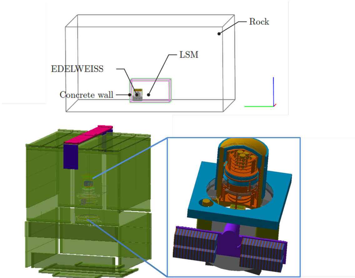
Figure 3.12. – Visualization of the EDELWEISS-III geometry as implemented in the simulation code. The \mu -veto system, with the newly implemented modules covering the gap between the two chariots, and the cryostat together with the warm electronics are shown.
