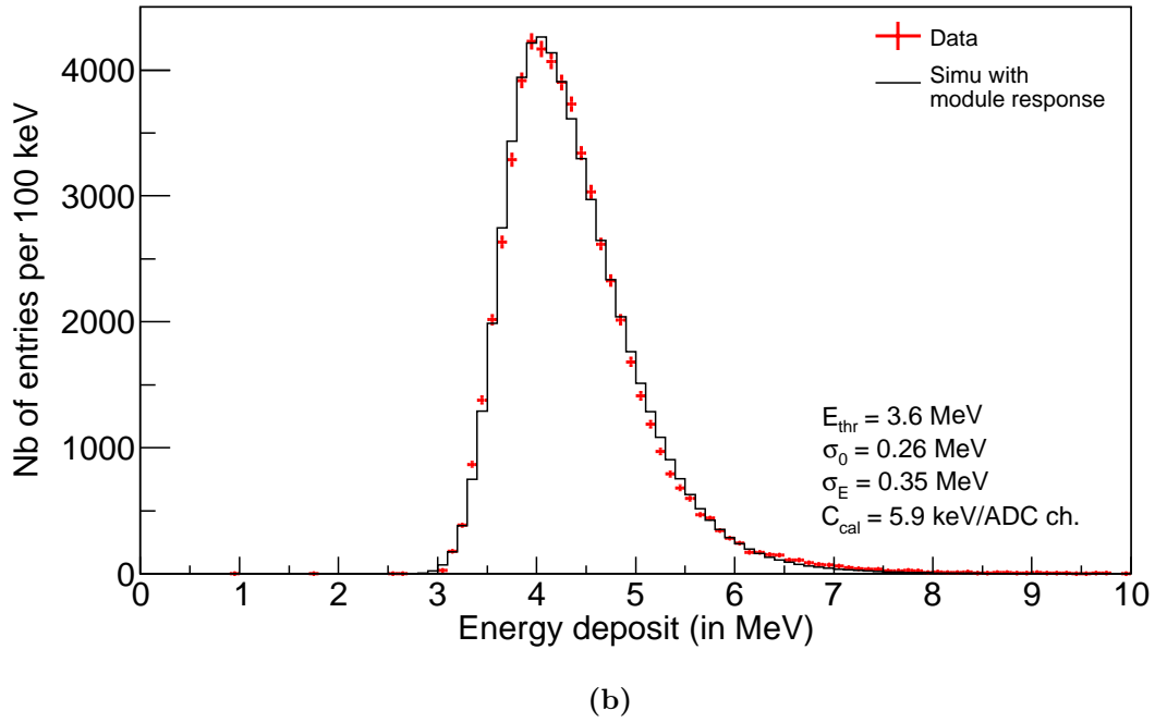
Figure 4.20. – Energy distributions of the AmBe source located at the center of module M42. The red markers shows the measured energy spectrum. The black histogram shows the simulated energy spectrum including the module response, obtained using the set of parameters giving the best match with the measured spectrum (written in the right bottom corner).
